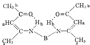
PROTON RESONANCE DATA FOR BIS-(ACETYLACETONE) SCHIFF BASES IN P.P.M. RELATIVE TO TETRAMETHYLSILANE
