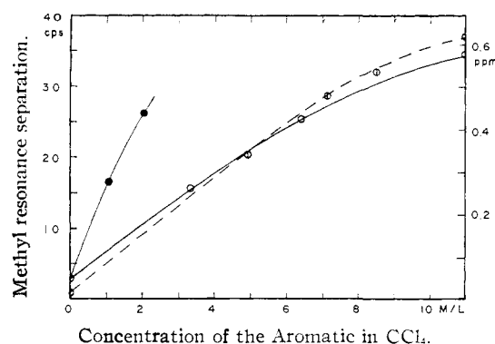
Fig. 3.—The dependence of \Delta\text{CH}_3 ( cf. Table III) on concentration of the aromatic solvent. Solid lines refer to bis-(acetylacetonate)-ethylenediimine and dotted lines to bis-(acetylacetonate)-tetramethylenediimine: ●, naphthalene in \text{CCl}_4 ; ○ and ◊, benzene in \text{CCl}_4 (zero M is pure \text{CCl}_4 , 11 M is pure benzene).
