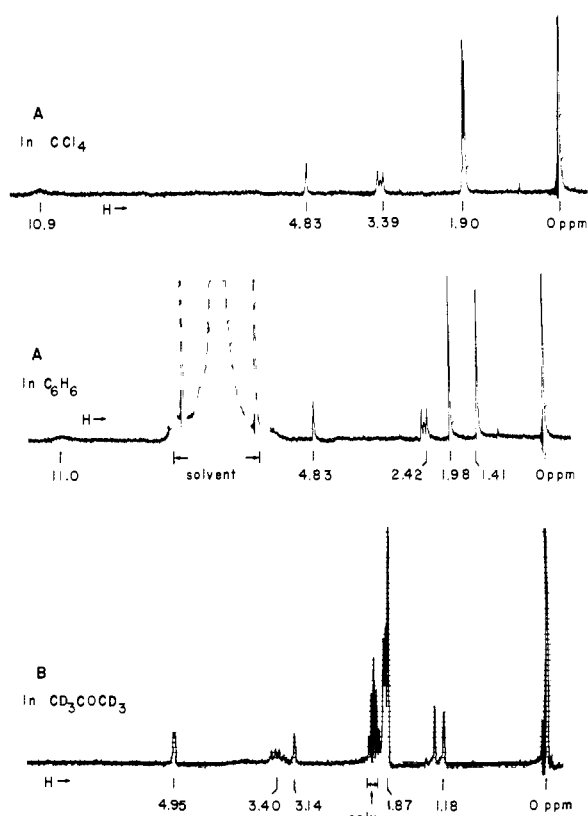
Fig. 1.—Proton spectra (at 60,000 Mc.) of: A. bis-(acetylacetonate)-ethylenediimine and B bis-(acetylacetonate)-propylenediimine (in B, the low field signal at 10.8 p.p.m. is omitted).
