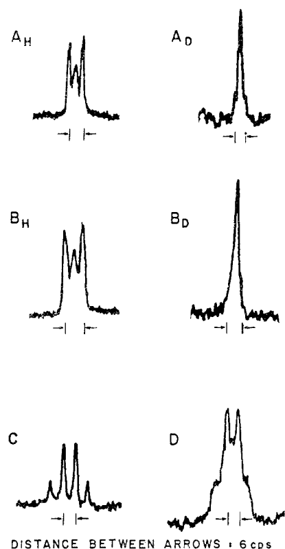
Fig. 2.—The methylene bridge signals (near 3.4 p.p.m.) of the diimines: A_H , bis-(acetylacetonate)-ethylenediimine, A_D , the same compound monodeuterated; B_H , diethyl-(ethylenebis- \beta -aminocrotonate), B_D , the same compound monodeuterated; C , bis-(acetylacetonate)-trimethylenediimine; D , bis-(acetylacetonate)-tetramethylenediimine.
